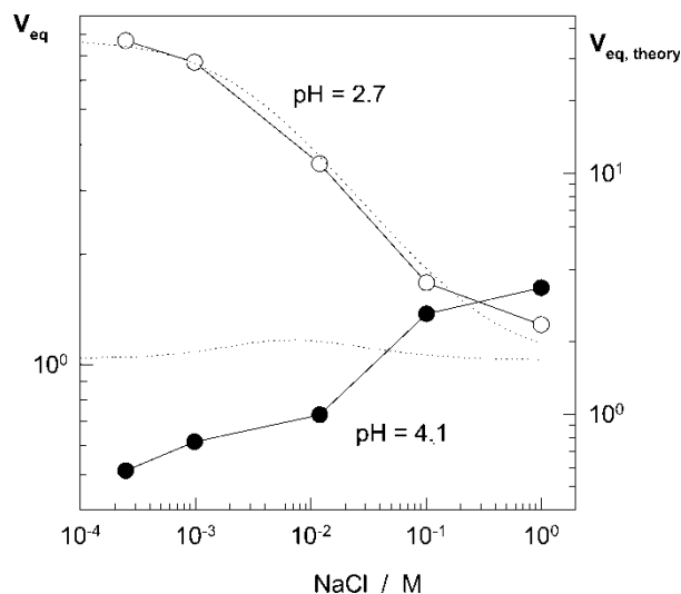
Figure 6. The experimental swelling curves (solid lines) of 10/20-gels at pH = 2.7 and 4.1 in NaCl solutions of varying concentration are shown in comparison with the predictions of the theory (dotted curves). The gel volume calculated using the theory ( V_{eq,theory} ) was adjusted to fit the experimental V_{eq} data obtained at pH = 2.7.
