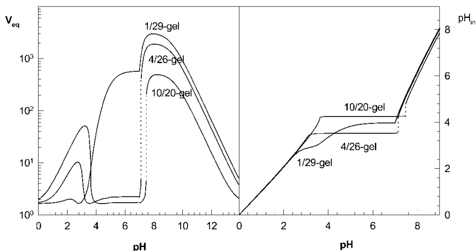
Figure 5. The equilibrium volume V_{eq} of the hydrogels with three different molar ratios of MAPTAC/AAC units and pH in the gel solution ( pH_{in} ) shown as a function of pH of the external solution. Phase transition regions are indicated by the vertical dotted lines. Calculations were using Equations (13) and (15).
