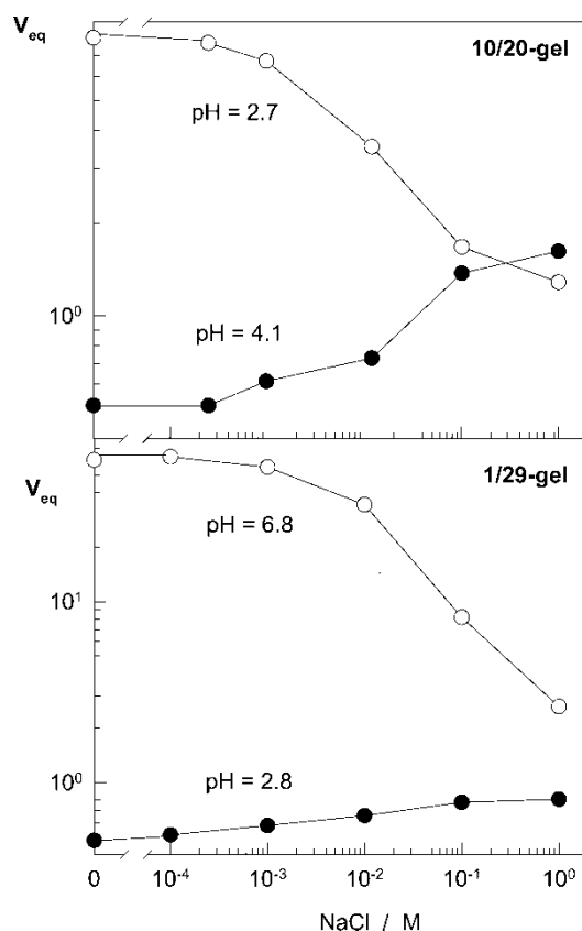
Figure 4. The equilibrium volume V_{eq} of 10/20-gels (upper Figure) and 1/29-gels (lower Figure) plotted against the concentration of NaCl solution. pH of the external solutions are indicated.
