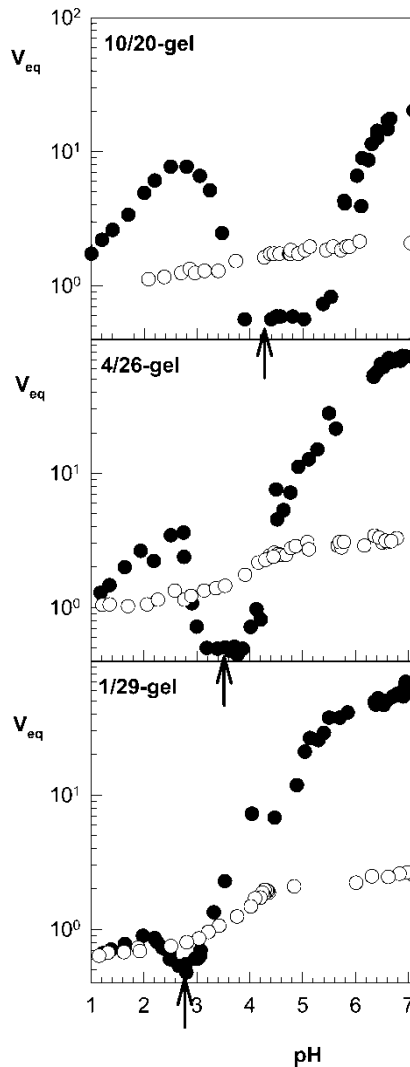
Figure 3. The equilibrium volume V_{eq} of the hydrogels with three different molar ratios of MAPTAC/AAc units shown as a function of pH of the external solution. Filled symbols are the results of measurements in water while open symbols are those measured in concentrated (1 M) NaCl solutions. The arrows in the Figures indicate pH_{cr} values of the hydrogels calculated using Equation (5).
